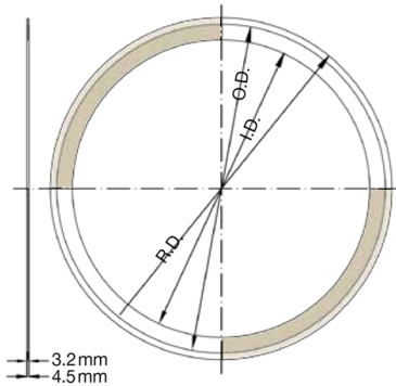
DIMENSION ACCORDING TO ASME B 16.20 FOR FLANGE ASME B 16.5 CLASS 150lb
